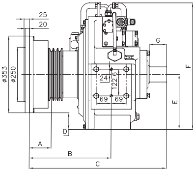
S Type Directly Mount
