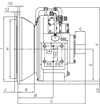
H Type Bell Housing
